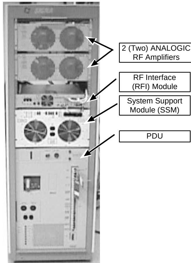
1.5T RF/PDU CABINET LOCATIONS ILLUSTRATION 1-1
