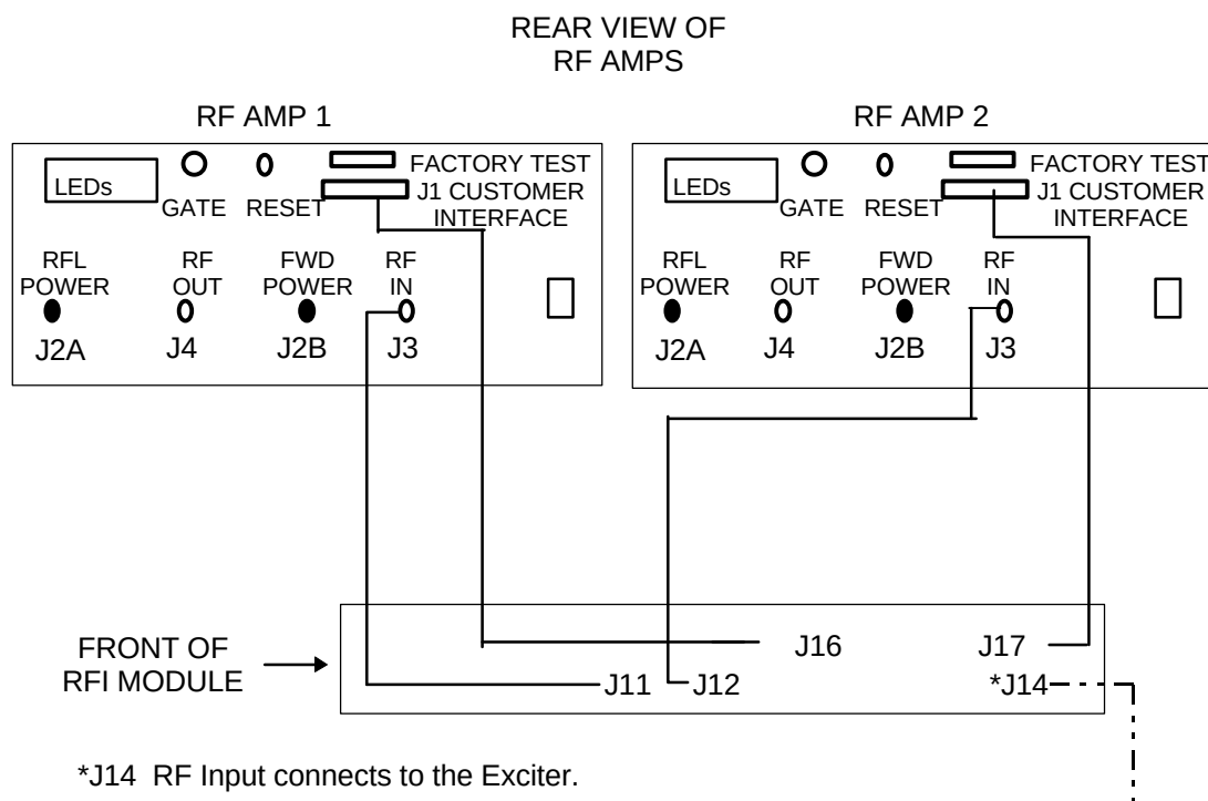
FRONT CABINET RF INTERCONNECTS ILLUSTRATION 2-2
