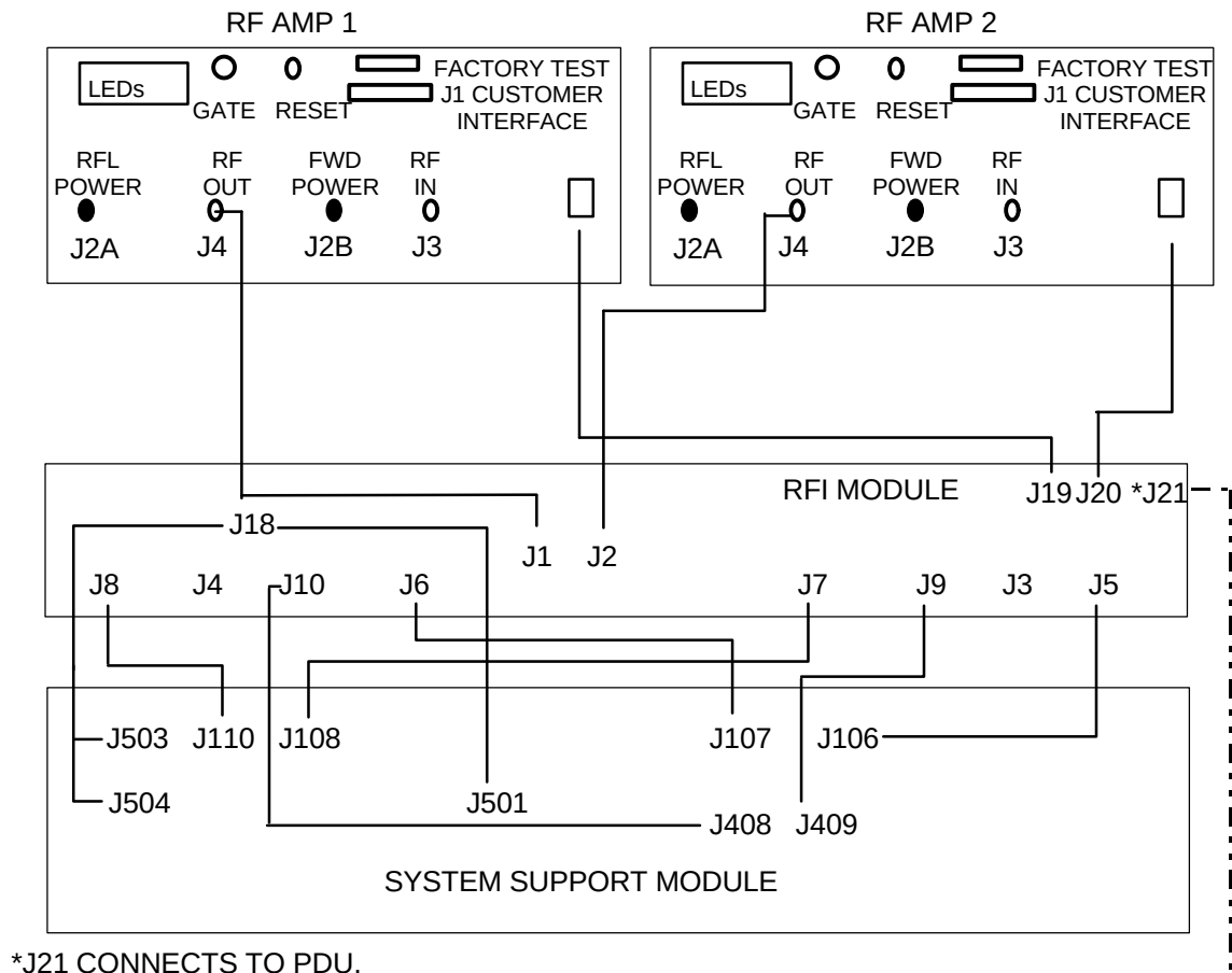
REAR CABINET RF INTERCONNECTS ILLUSTRATION 2-1
