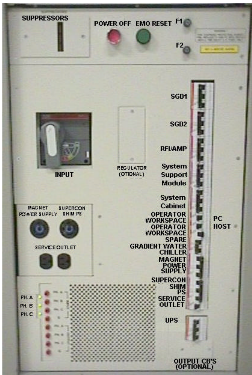
PDU FRONT DETAIL ILLUSTRATION 1-11
