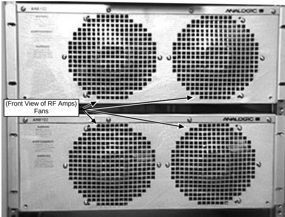
1.5T RF AMP FAN LOCATION ILLUSTRATION 1-8
